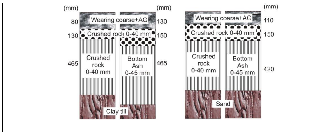
Figure 4-3. Illustration of materials used in road construction in Törringe (left) and Dåvamyrän (right). For each site, the reference structure is shown on left, test structure on right. Bottom ash is used as a subbase course in the test structure, overlain by crushed rock in the base course. AG = asphalt-bound gravel
